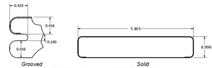
Figure 12 - Fiberon Paramount® PVC Cross-Section
