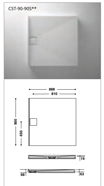
** Side Drainhole
