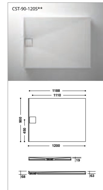
** Side Drainhole
